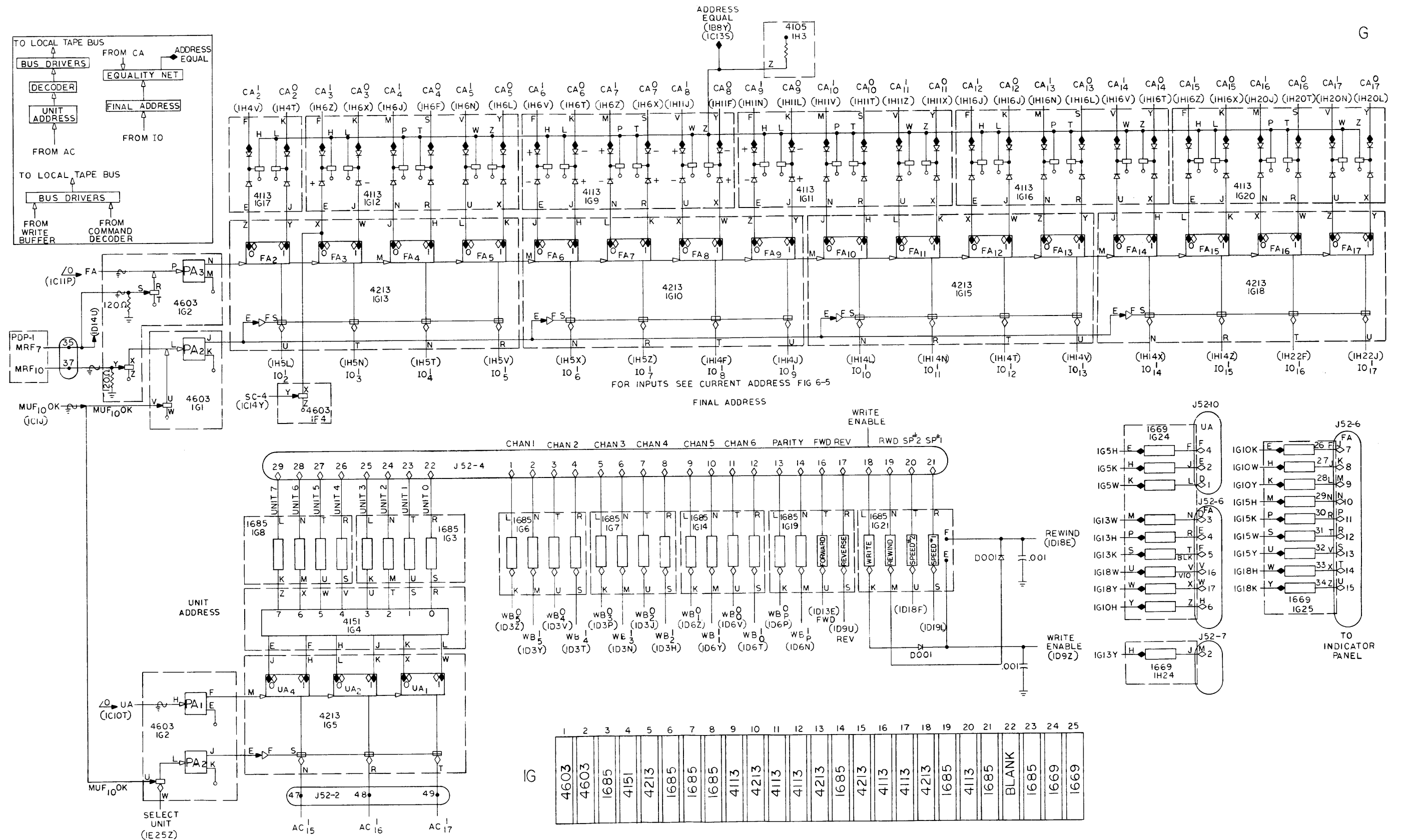
Figure 6-12 Unit, Final Address, Address Equal
