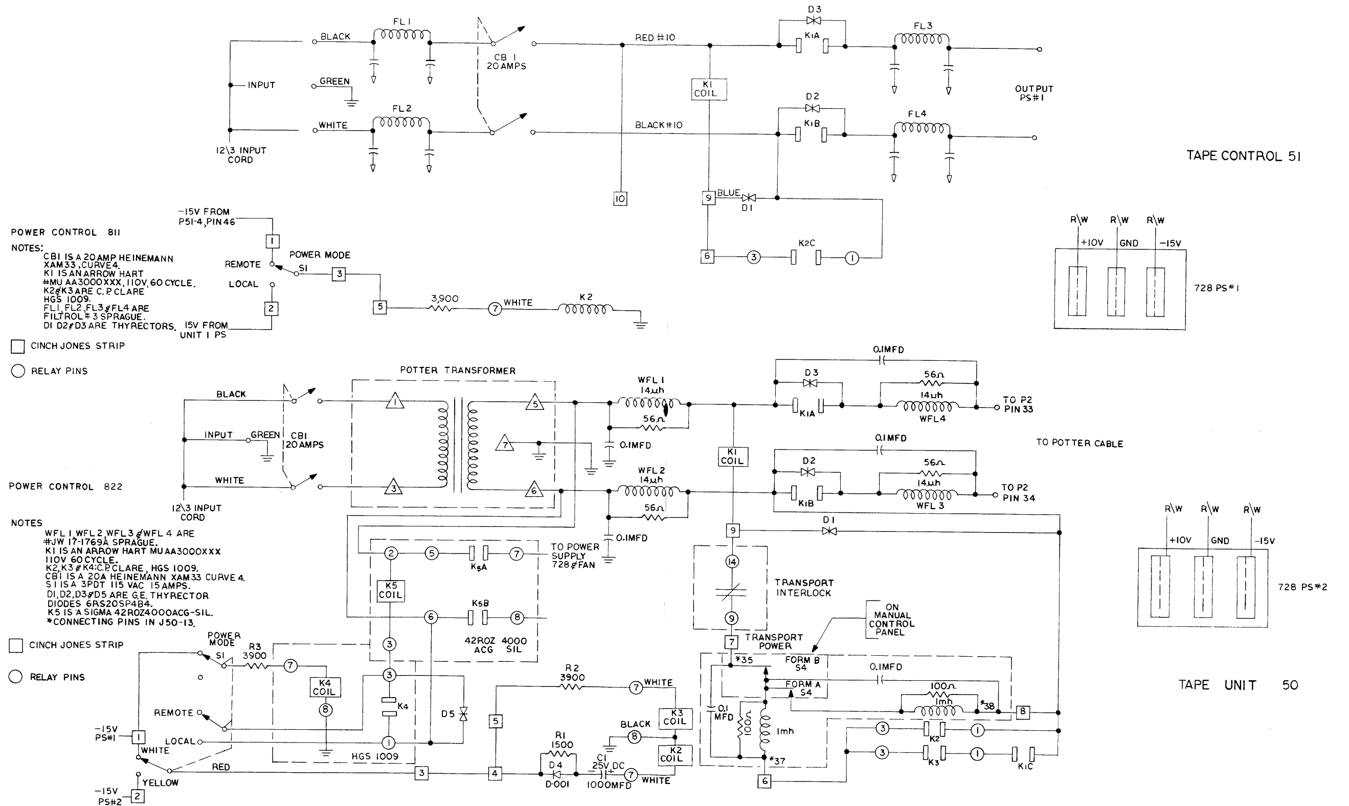
Figure 7-1 Power Control Wiring for Types 50 and 51 Combination
