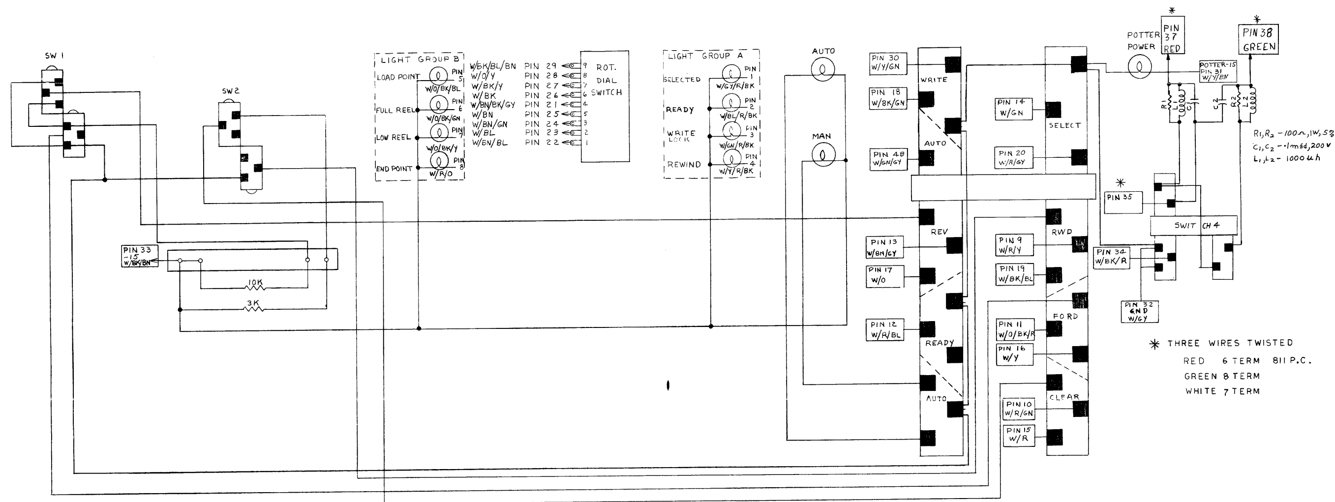
CABLE SCHEDULE FOR 50 PIN AMPHENOL CONNECTOR
