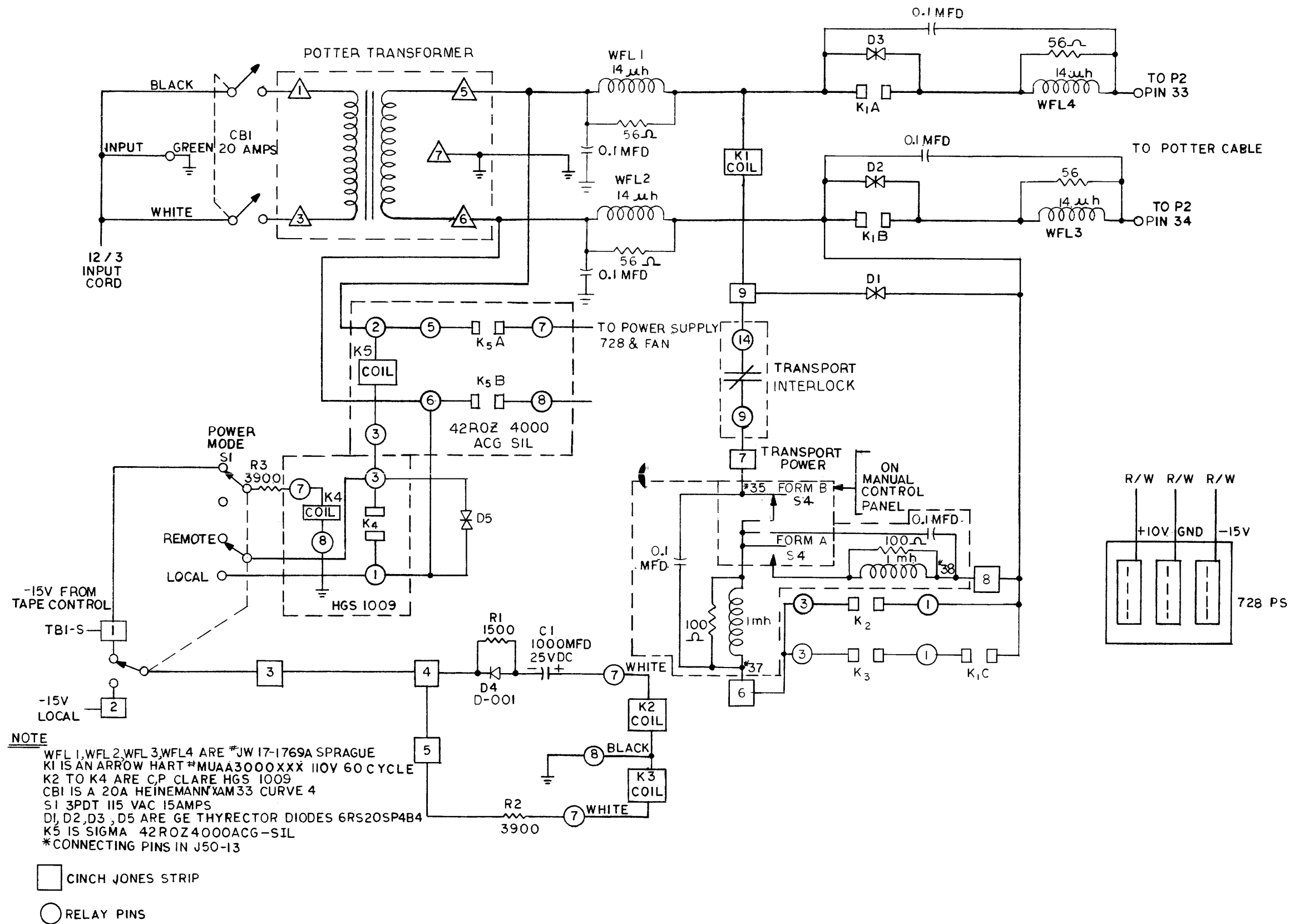
Figure 7-3 Power Control Wiring for Tape Unit 50
