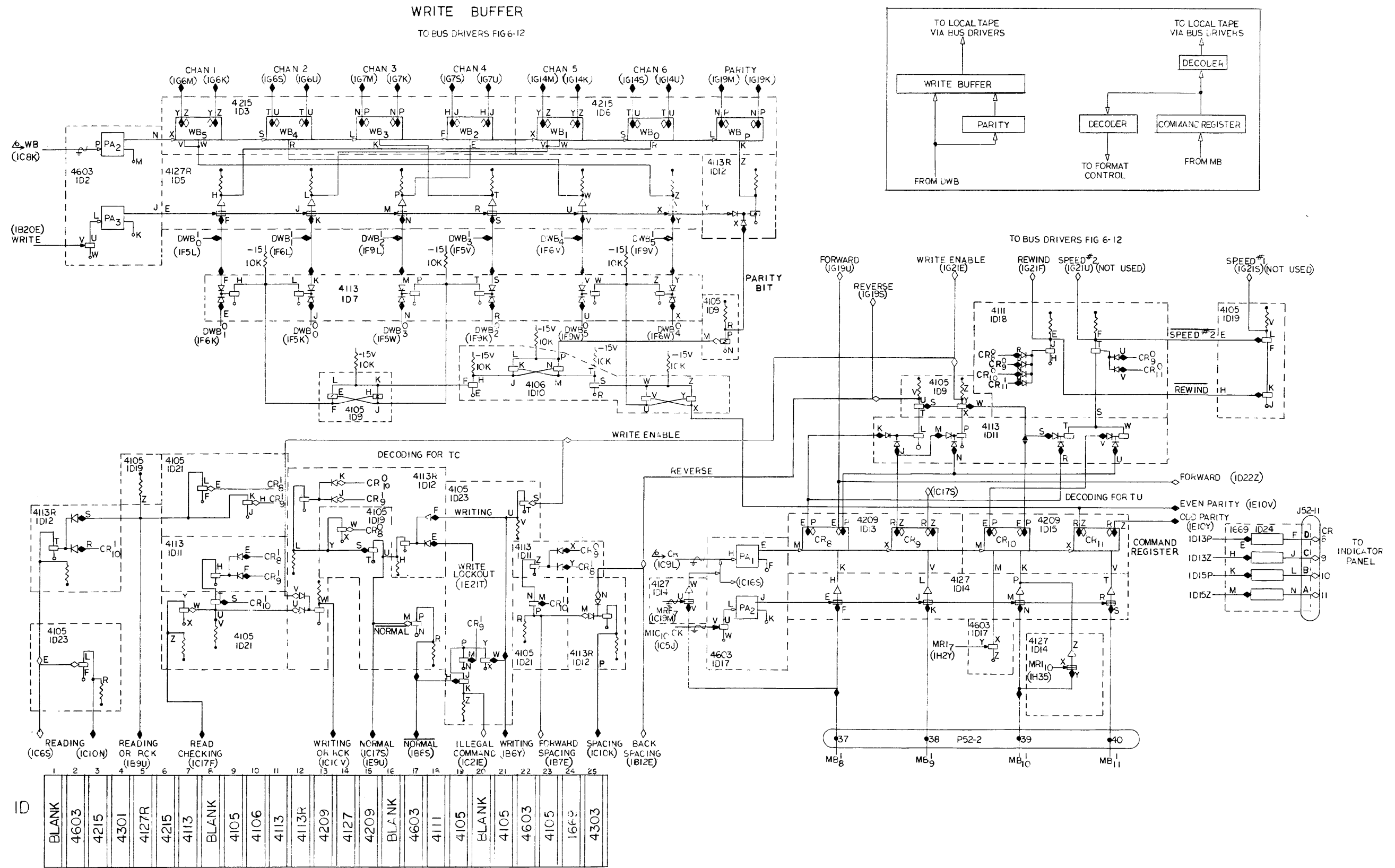
Figure 6-10 Command Register, Command Decoders, Write Buffer
