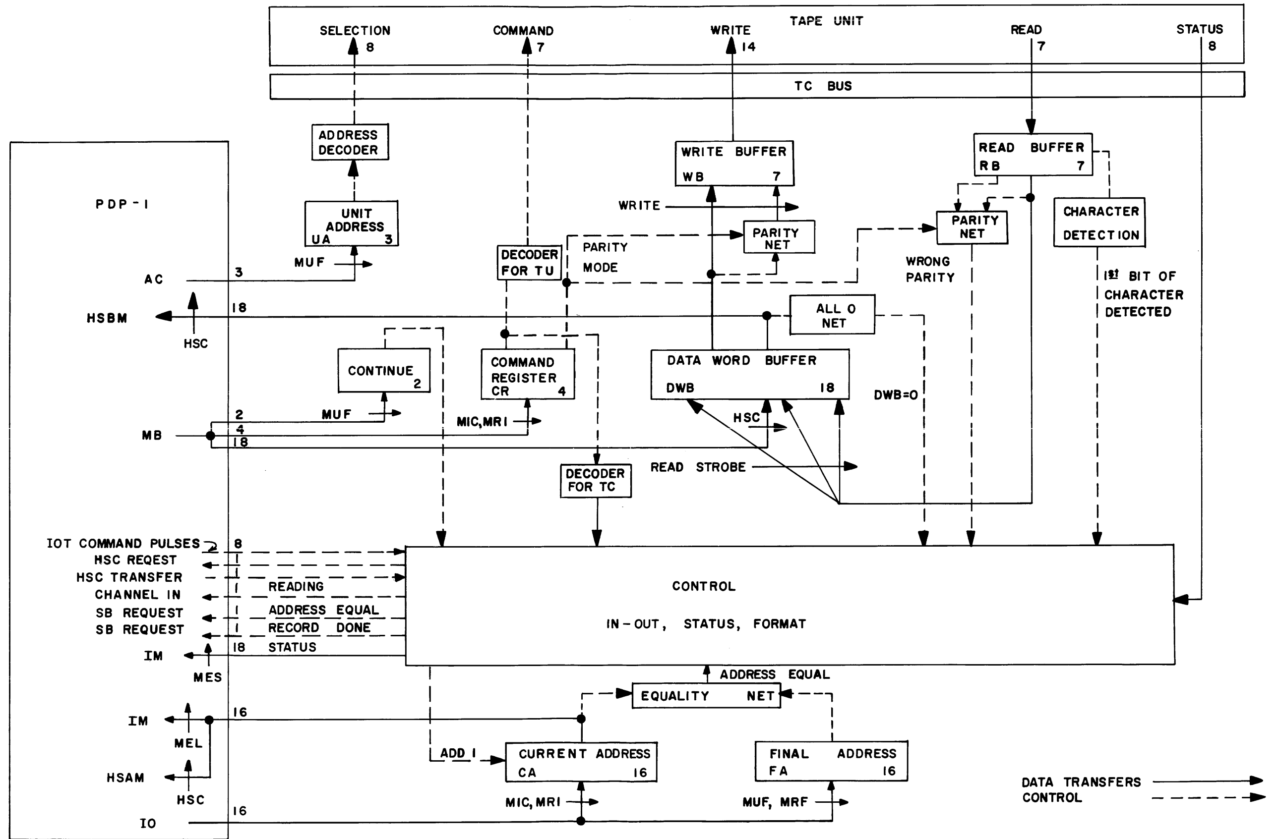
Figure 4-4 Automatic Tape Control 52 Block Diagram
