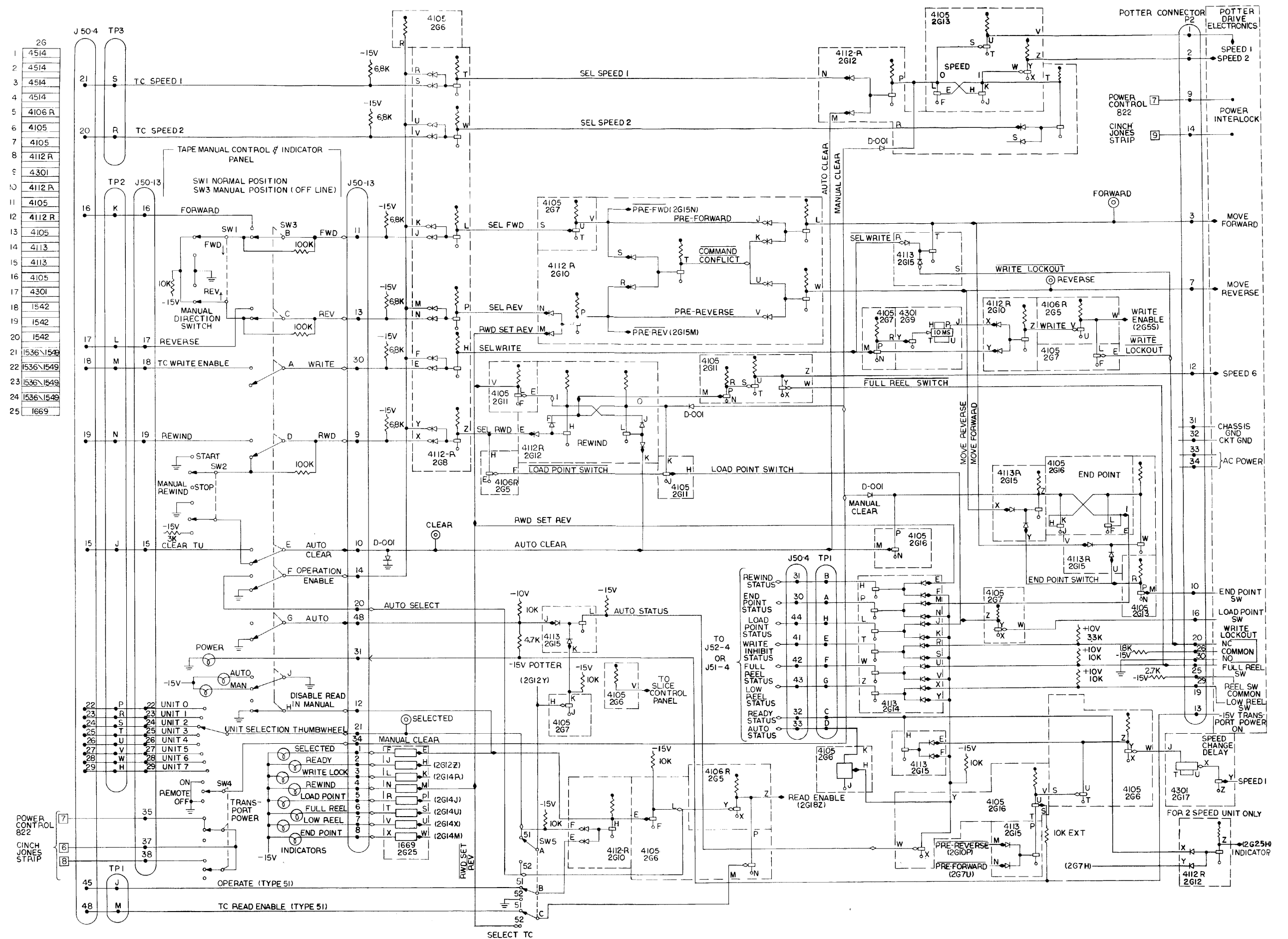
Figure 6-18 Tape Unit 50: Transport Logic
