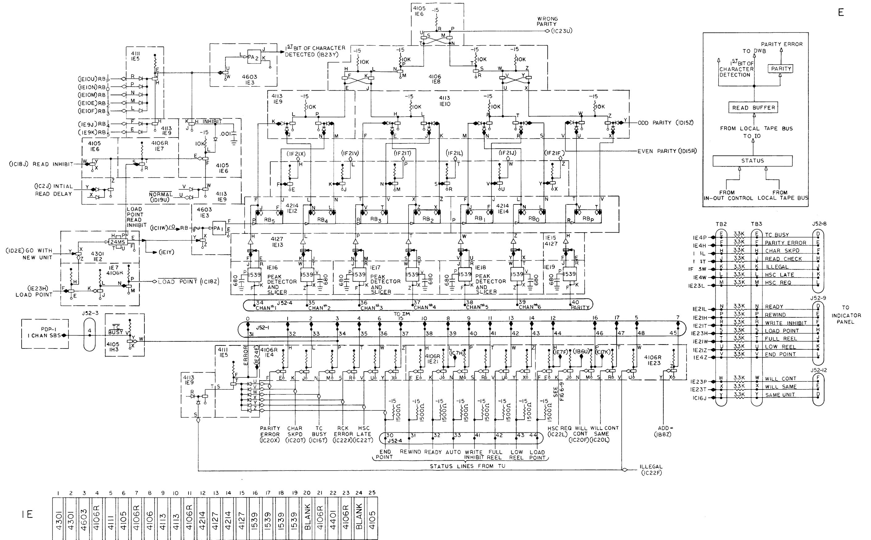
Figure 6-14 Read Buffer, Status
