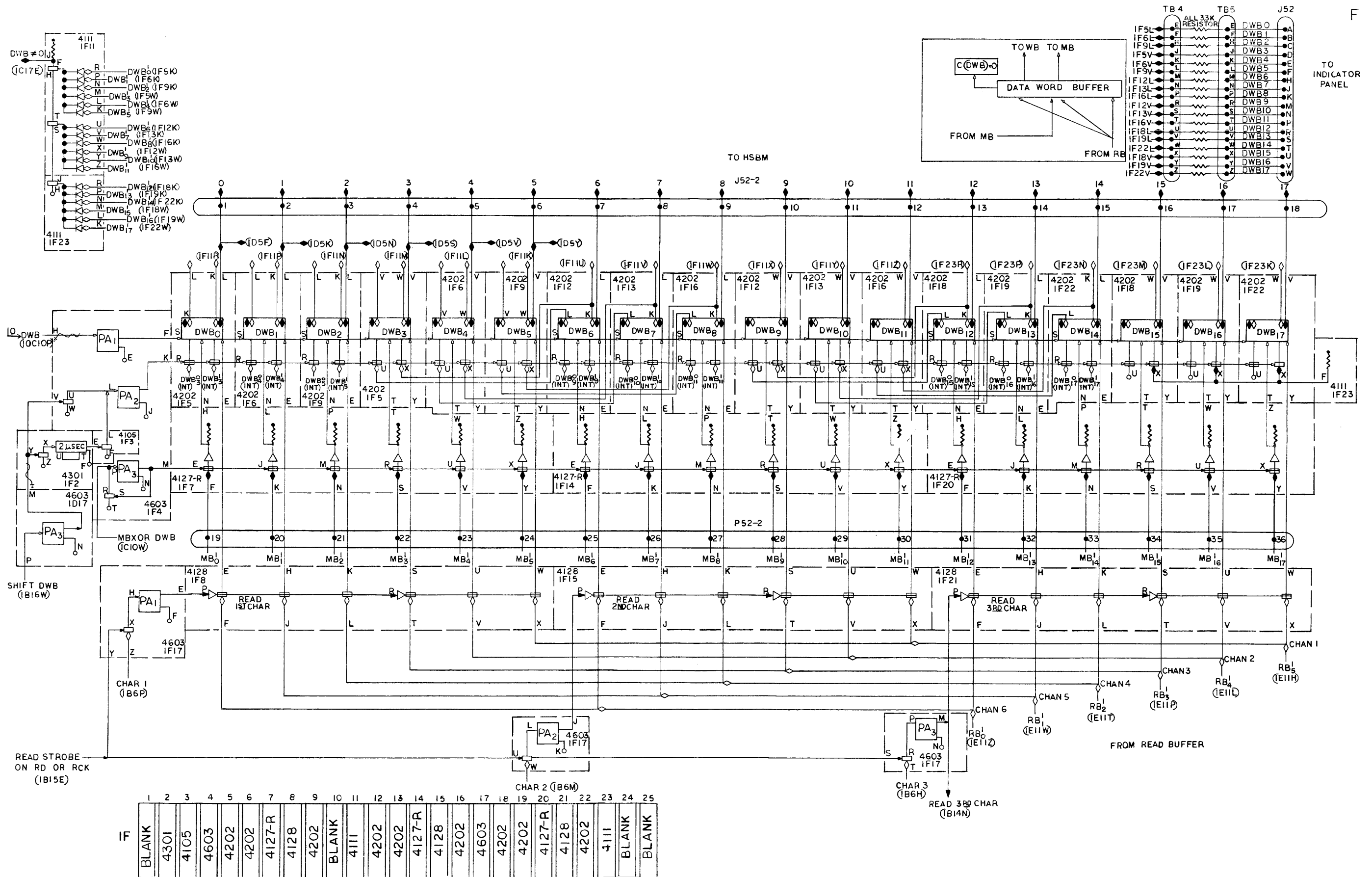
Figure 6-13 Data Word Buffer
