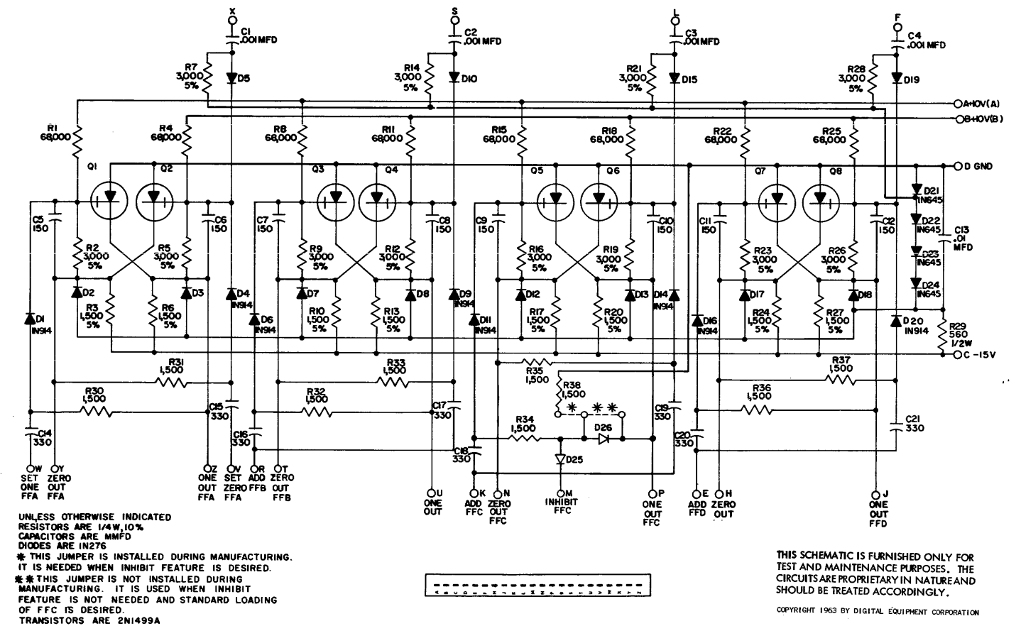
Four-bit Counter 4215
