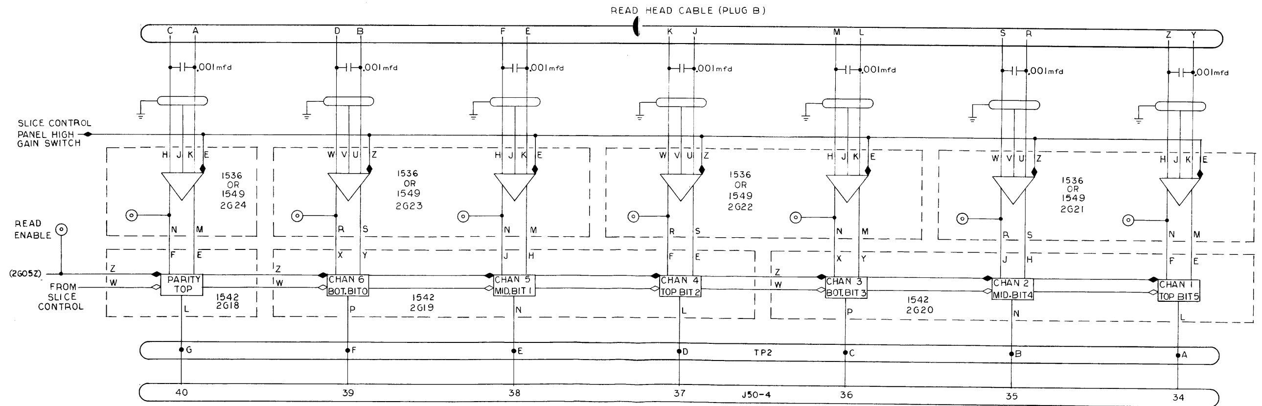
Figure 6-19 Tape Unit 50: Read-Write Circuits
